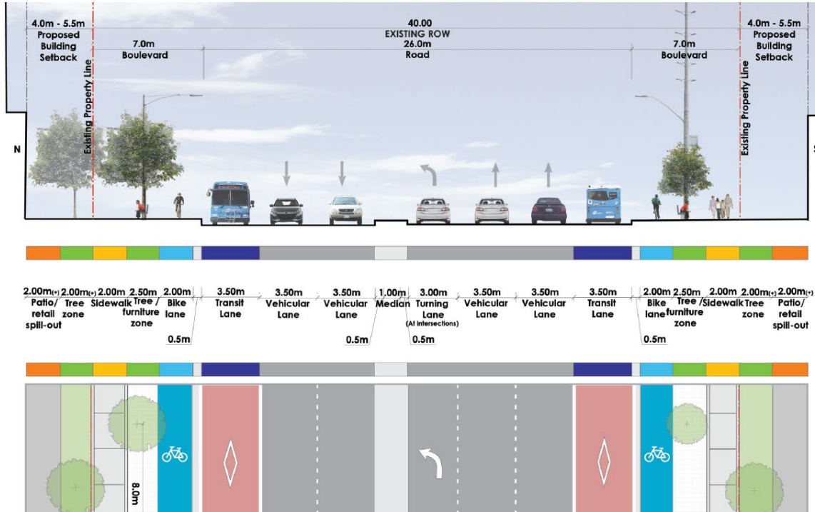
Figure 3.7: Curbside BRT configuration
