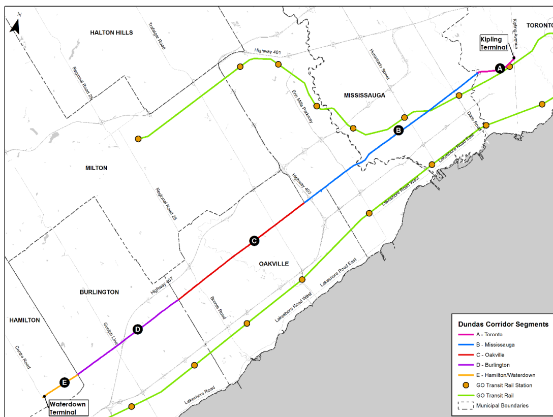
Figure 1.1: Dundas Corridor Segmentation
